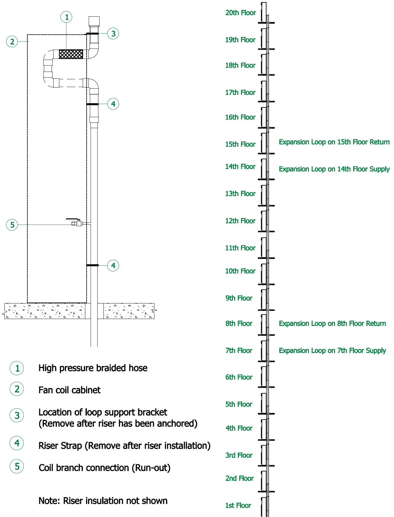
Figure 13: Riser Expansion
